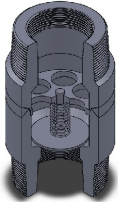
Figure 1: Valve Cutaway
